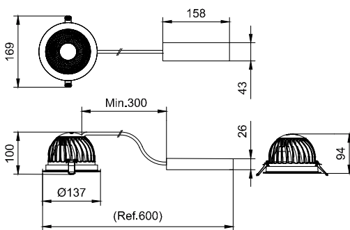
DN588B LED6/840 PSU C D125 C WH WB GM
